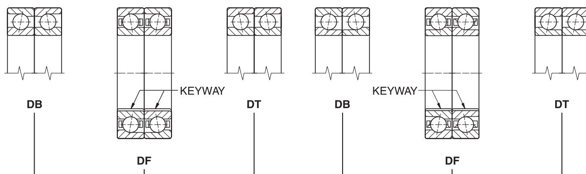
Old Design, MM-EX Bore and O.D. Tolerance Nominal + Tolerance "WT" Construction
