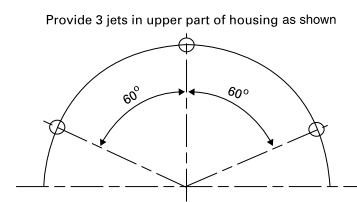
Fig. 4-36 Cooling jets in top part of the housing for speed above 25 m/s
