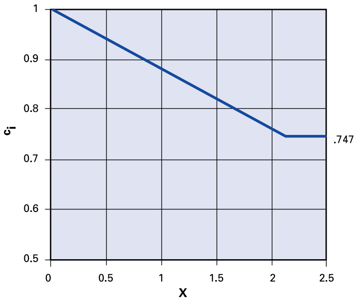
Figure 4-41b Load zone factor ( C_l ) for case-carburized bearings.
