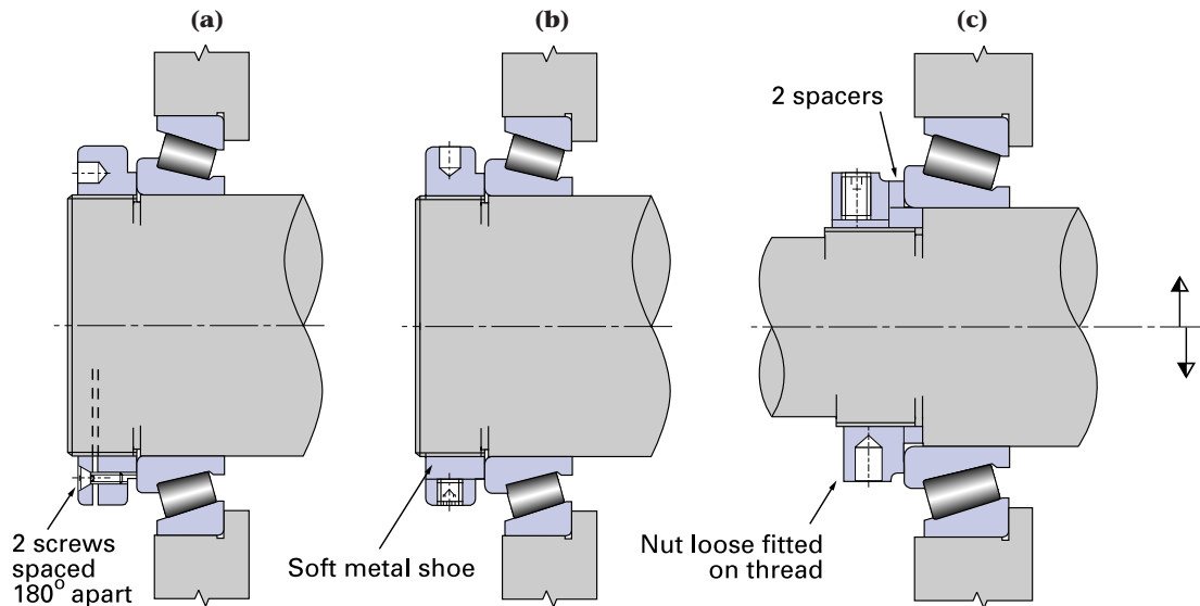
Fig. 4-12 Locking devices
