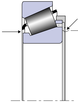
Fig. 4-37 The TSM bearing
