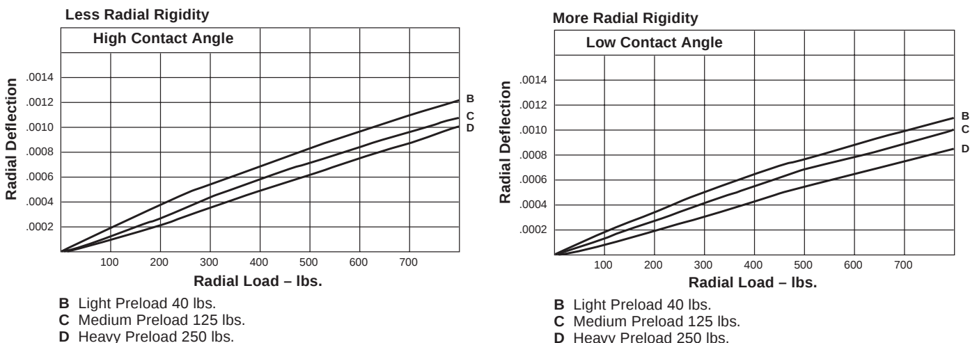
Figure 4-11 – Radial Deflections
