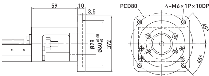
Adapter flange F7
