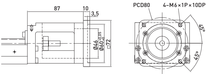
Adapter flange F9
