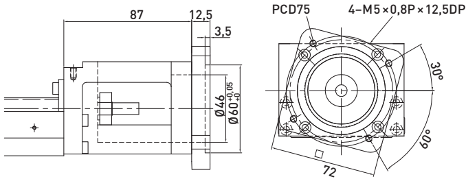
Adapter flange F8
