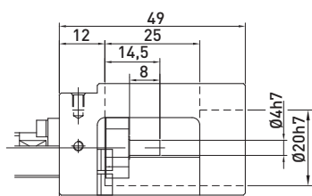
Adapter flange F0
